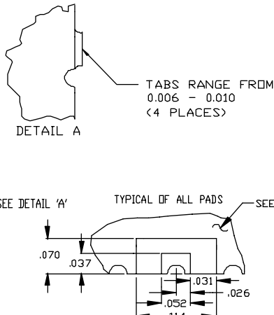
PHYSICAL DIMENSIONS
